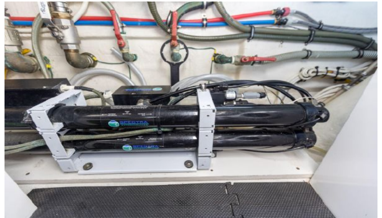
Water Maker
